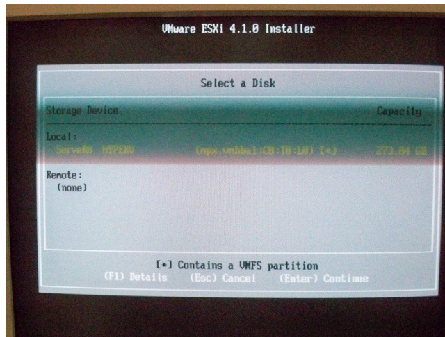
Select disk for the installation image
